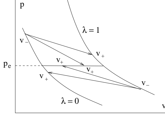
Figure 2 The points (v_{\pm}, \lambda_{\pm}) of liquefaction waves ( p_{\pm} \geq p_e ) and evaporation waves ( p_{\pm} \leq p_e ). The arrows point to the fronts of the waves.
