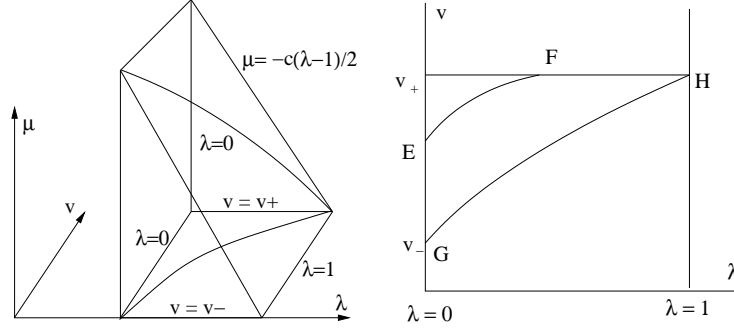
Figure 3 The pentahedron and the top view of its base \mathcal{F}_b . On the curve EF , p(\lambda, v) = p_e . On the isocline GH , v' = 0 .
