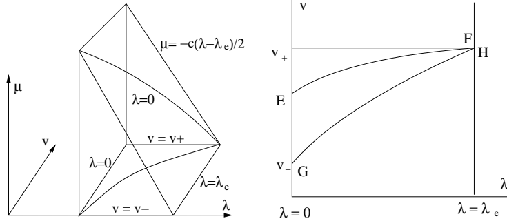
Figure 4 The pentahedron and the top view of its base \mathcal{F}_b . On the curve EF , p(\lambda, v) = p_e . On the isocline GH , v' = 0 .
