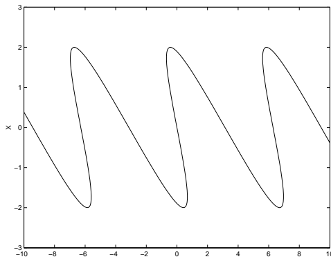
FIGURE 3.5. The cross section of the surface \mathcal{B} at k = 2 , after cusps have formed.
