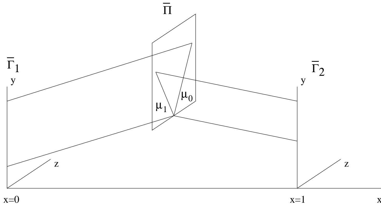
The transversal intersection of \mu_0 and \mu_1
