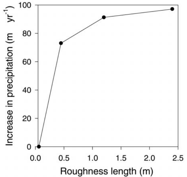
FIG. 6. Effect of roughness length on mean annual precipitation in tropical savanna. The graph shows the increase in precipitation resulting from an increase in roughness length relative to the grassland scenario. The northern African savannas, which showed little response, were excluded from this analysis.
