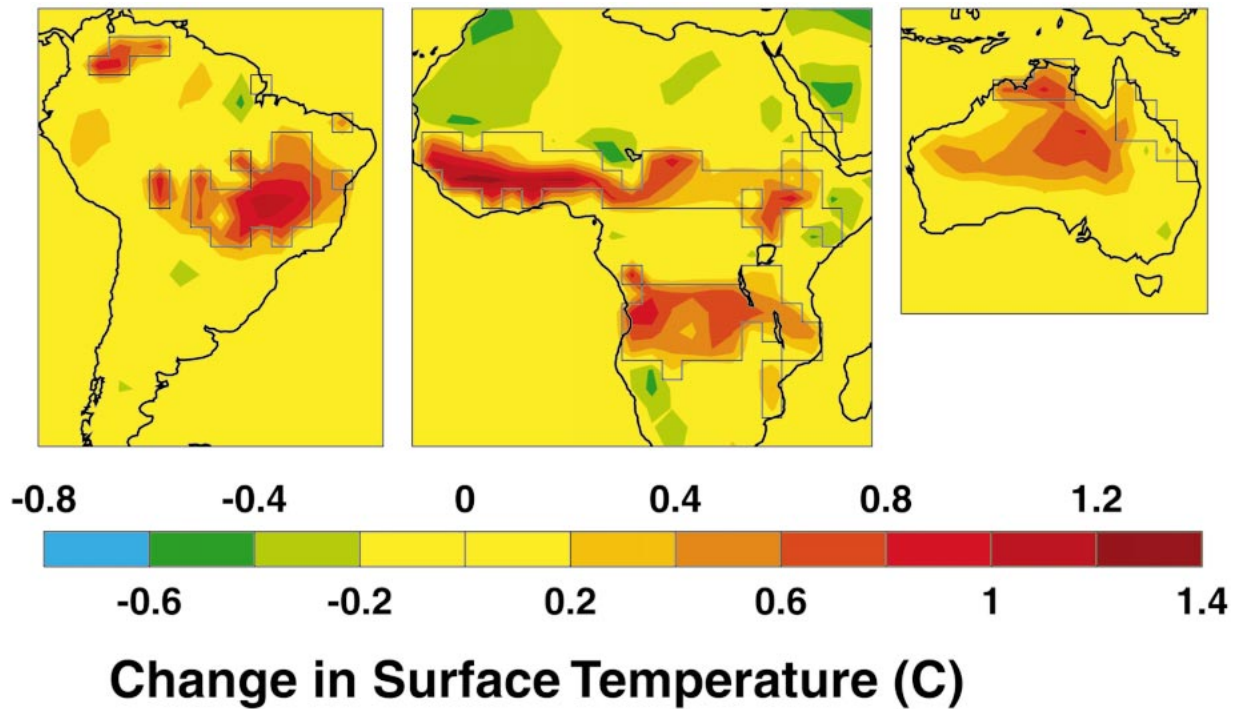
FIG. 3. Change in mean annual surface air temperature resulting from conversion of tropical savanna to grassland. All five savanna regions exhibited a significant increase in surface air temperature. Savanna regions are outlined.
