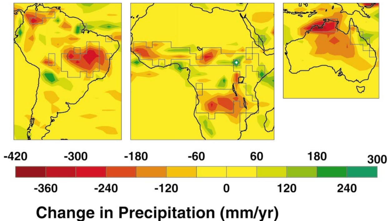
FIG. 2. Change in mean annual precipitation resulting from conversion of tropical savanna to grassland. All savanna regions, except for the northern African savannas, exhibited a significant decline in precipitation. Savanna regions are outlined.
