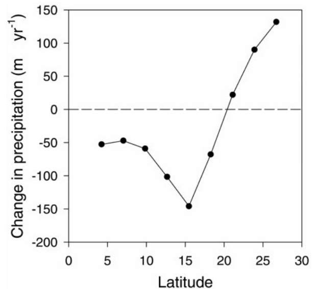
FIG. 7. The change in the latitudinal distribution of precipitation in the savanna regions resulting from a reduction in roughness length from 0.448 to 0.060. Savanna grid cells from the Northern and Southern Hemispheres were pooled to obtain a single mean for each latitude.
