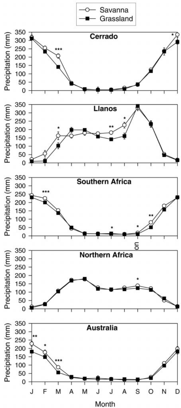
FIG. 4. Effect of savanna transformation on the seasonal pattern of precipitation. Significant differences are denoted by the symbols: * (0.05 < P < 0.01), ** (0.01 < P < 0.005), *** (P < 0.005).
