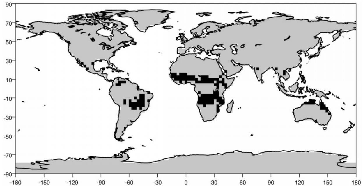
FIG. 1. The global distribution of tropical savannas, as used in this study. Five major savanna regions are defined here: northern South America, the Brazilian savannas, northern Africa, southern Africa, and northern Australia. Grid cells prescribed as savanna are darkened.
