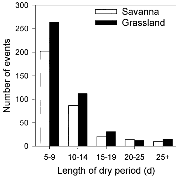
FIG. 5. Effect of savanna transformation on the frequency of dry periods during the summer wet season. Three years of simulation data were summed over the Southern Hemisphere savanna regions, for Jan–Mar. In the grassland scenario, the frequency of prolonged dry periods within the wet season was greater than in the savanna scenario.
