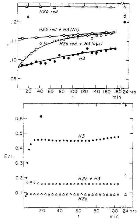
FIGURE 8: (A) Fluorescence anisotropy of H2b reduced (Δ), H3 (●), and H2b reduced plus H3 observed (○) and calculated for a mixture of noninteracting (NI) proteins (□), as a function of time after adding phosphate. (B) Light scatter of H2b reduced (Δ), H3 (●), and H2b reduced plus H3 (○) as a function of time after adding phosphate. Buffer conditions are as described in the text. Concentrations of individual proteins are 1.0 \times 10^{-5} and 1.0 \times 10^{-5} M each in the mixed solutions.
