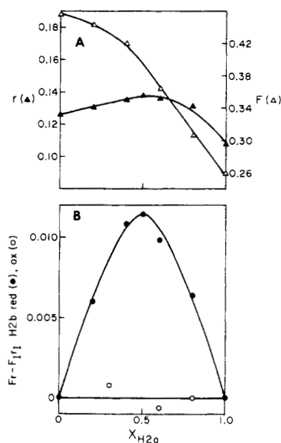
FIGURE 5: Fluorescence continuous variation curves of histone H2a plus H2b. (A) Anisotropy ( \blacktriangle ) and intensity ( \triangle ) of H2a, H2b reduced mixtures. (B) F_r - F_{r1} for H2a plus H2b reduced ( \bullet ) and H2a plus H2b oxidized ( \circ ). For all curves buffer conditions are as given in the text. C_0 = 1 \times 10^{-5} M. The subscript 1 denotes values calculated for noninteracting mixtures.
