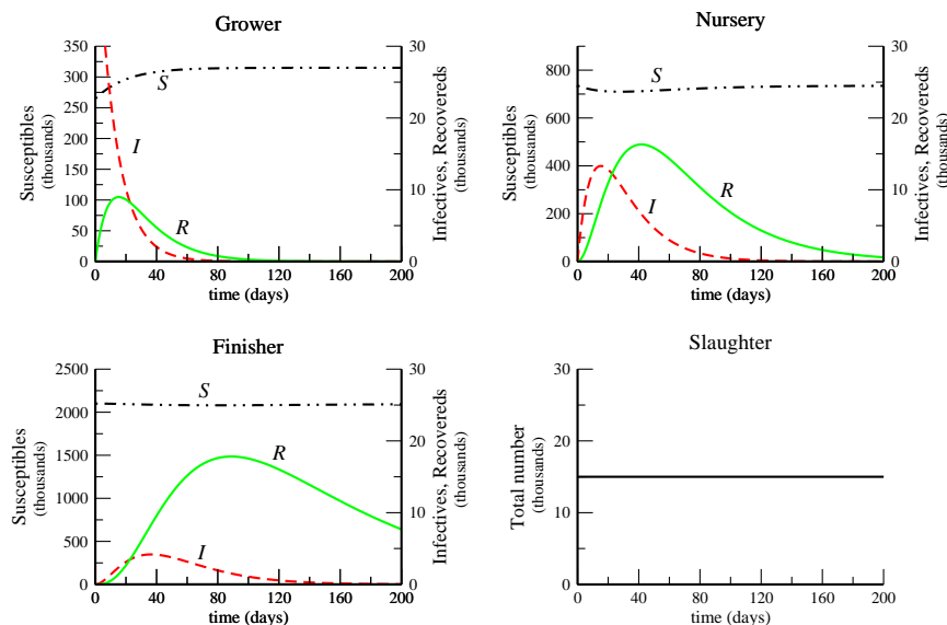
FIGURE 10. Simulation I: Recovery and movement of infectious individuals through the network, in the absence of transmission. Notice that susceptible numbers are plotted on different scales (left vertical axis on each panel) from infective and recovered numbers (right vertical axis on each panel). Parameter values are given in the text: each \beta_i is set equal to zero, infection is assumed to last 31 days and immunity lasts 180 days. The initial conditions are N_1 = 315,000 , N_2 = 735,000 , N_3 = 2,100,000 and N_4 = 15,000 . Of the piglets at the first node, 50,000 are initially taken to be infectious, while the remainder of the population is susceptible.
