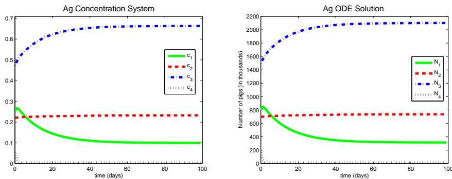
FIGURE 4. Numerical solution of the deterministic (rate equation) system (9) for t \in [0, 100] . Parameter values are as given in Table 3.
