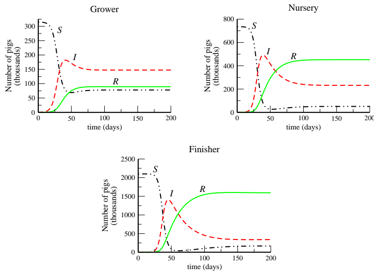
FIGURE 11. Simulation II: Dynamics following the introduction of infection, with R_0 = 10 . This value of the basic reproductive number determines the value of the transmission parameters ( \beta_i ). Initial conditions and other parameter values are as in the previous figure, except that only 200 of the 315,000 individuals at the grower node are infective at the initial time.
