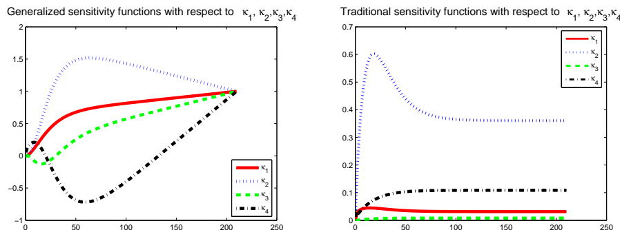
FIGURE 7. Generalized and traditional sensitivity functions for \kappa_1 , \kappa_2 , \kappa_3 , \kappa_4 , employing a simulated data set with M = 210 , generated as discussed in the text. Underlying parameter values are \kappa_1 = 1.674 , \kappa_2 = 0.322 , \kappa_3 = 4.521 , \kappa_4 = 1 , while all other parameters are as given in Table 3.
