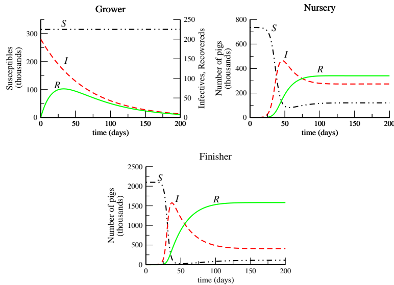
FIGURE 12. Simulation III. Age-dependent transmission of infection. If there were no transportation of animals, the basic reproductive numbers at the grower, nursery and finisher nodes would equal 2, 10 and 15, respectively. These values of R_0 determine the parameters \beta_1, \beta_2 and \beta_3 . All other parameter values and initial conditions are as in the previous figure. For the panel depicting the grower, note that susceptible numbers are plotted on a different scale (left vertical axis) from the infective and recovered numbers (right vertical axis), and these infective and recovered numbers are not in thousands. Also note that infection goes extinct in the grower node while a positive equilibrium level of infection is achieved at the nursery and finisher nodes.
