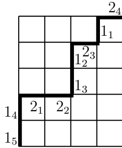
Figure 1: A partition \lambda contained in 5 \times 4 and the corresponding lattice path
