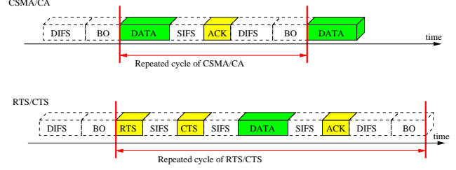
Figure 3. Timing diagram for CSMA/CA and RTS/CTS
