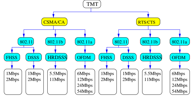
Figure 1. TMT classification based on different MAC and PHY schemes and basic data rates
