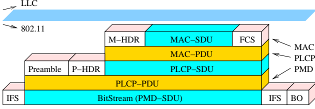
Figure 2. Overhead at different sublayers of IEEE 802.11
