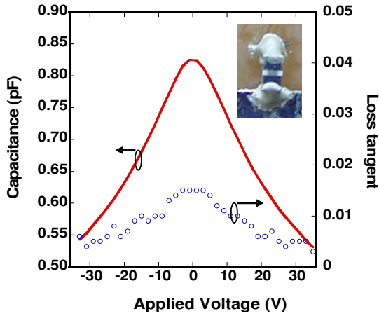
Fig. 2: Representative C-V characteristics of a BST interdigital varactor measured after dicing at 1 MHz.
