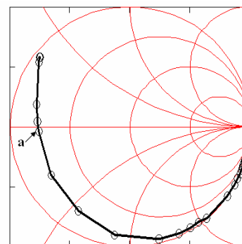
Fig. 1: Junction varactor reflection coefficient versus swept bias from -30V to +1V. Point (a) on the chart represents 570 mV forward bias. The measurement frequency is held constant at 50 MHz.
