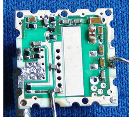
Fig. 4: Microstrip VCO shown with tune line input on the right output power obtained from matching transmission line on left. The BST varactor is located in upper right corner.
