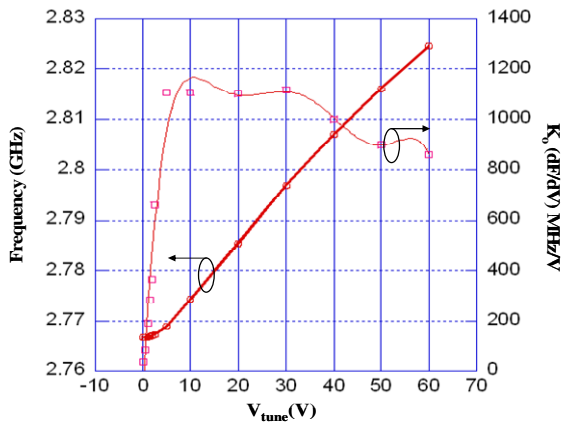
Fig. 3: Measurement of tune frequency and K_o versus tuning voltage
