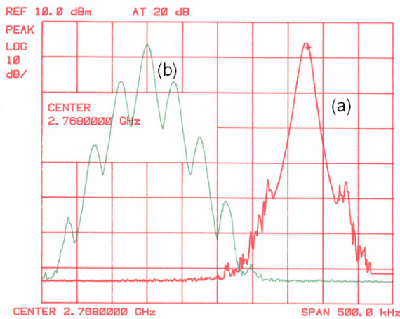
Fig. 8: Significant drop in loop gain due to K_o reduction causes larger noise peaking (a) and eventually instability (b).
