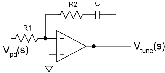
Fig. 5: Active loop compensator produces a second order type II PLL used in this study.
