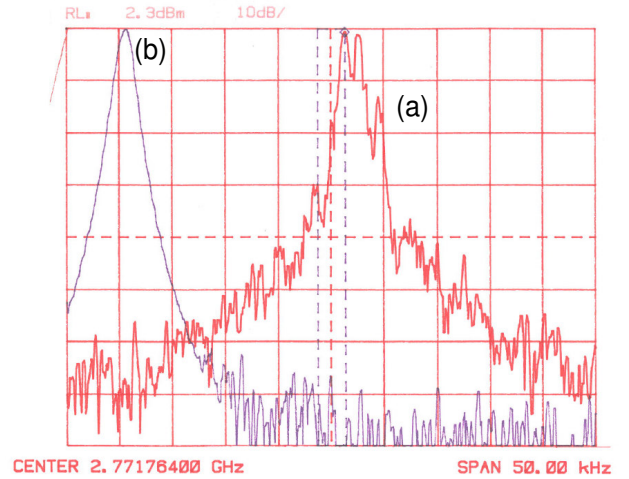
Fig. 6: The uncorrected noise (a) is suppressed in the tracking wide loop when properly damped for the loop gain and has no noise peaking (b).
