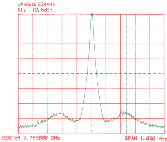
Fig. 7: Adjustment in the loop compensator permits noise peaking and assist in monitoring the loop gain variation by monitoring the power spectrum.
