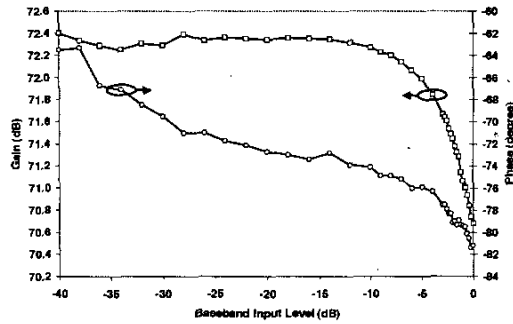
Figure 4: Measured superhet AM-AM, AM-PM at 1880MHz.
