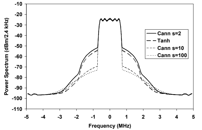
Fig. 2 Power spectrum at 2 dBm with complex Gaussian input signal.
