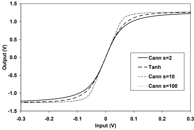
Fig. 1 Carrier transfer characteristic for limiter models.
