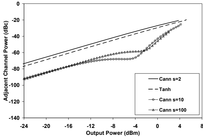
Fig. 3 Real Gaussian ACPR sweep.
