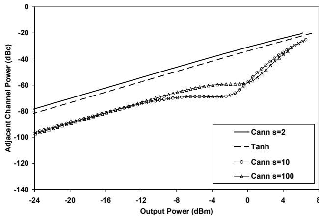
Fig. 4 Complex Gaussian ACPR sweep.
