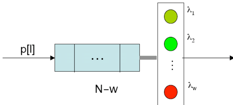
Fig. 4. The discrete-time output queue analyzed in isolation: finite capacity, w servers, slotted bulk arrivals.
