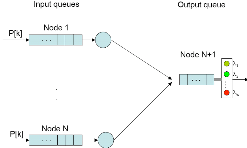
Fig. 2. The discrete-time queueing network with blocking
