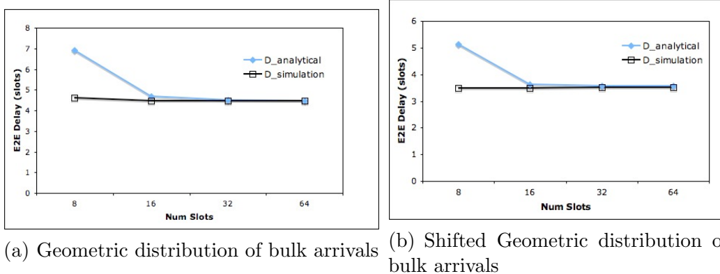
Fig. 6. Average end-to-end burst delay vs. number of slots s , N = 16 , k_{max} = 4 , d = 2 .
