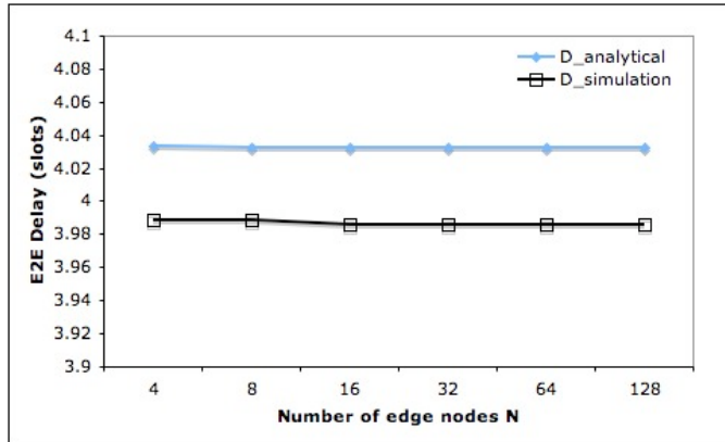
Fig. 8. Average end-to-end burst delay vs. number of edge nodes N in aggregation period T . Uniformly distributed bulk size, s = 32 , k_{max} = 4
