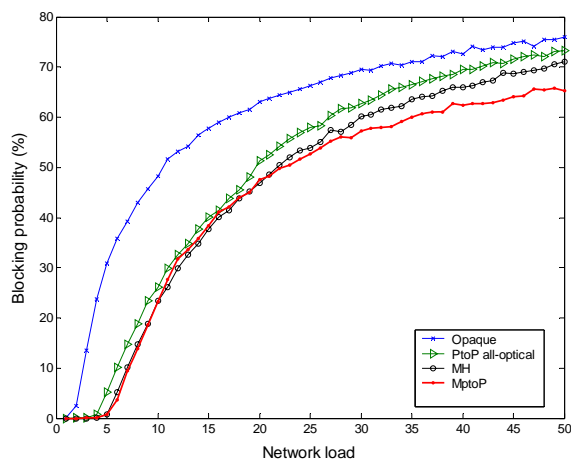
Fig. 21. Blocking probability evolution with the network load.
