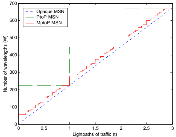
Fig. 13. The number of required wavelengths in the MSN network.
