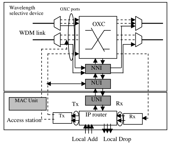
Fig. 11. Optical node architecture.
