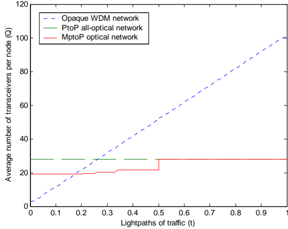
Fig. 17. The transceiver requirement per node in the US backbone.
