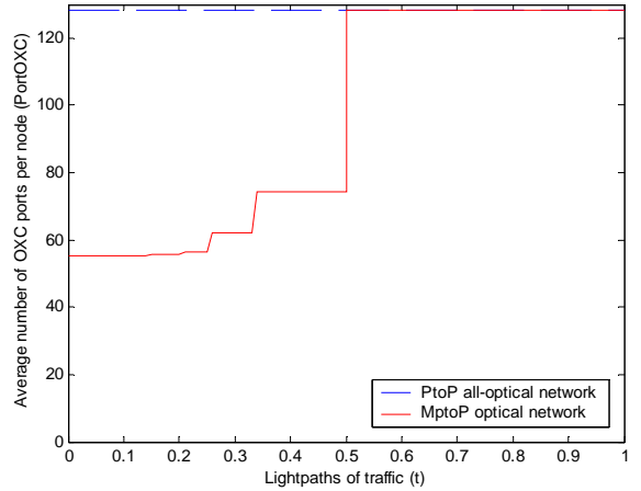
Fig. 18. The OXC port requirement per node in the US backbone.
