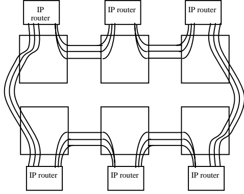
Fig. 5. An opaque WDM ring with three wavelengths.
