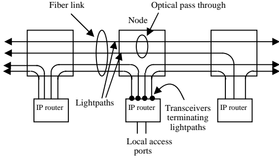
Fig. 4. A WDM ring node.
