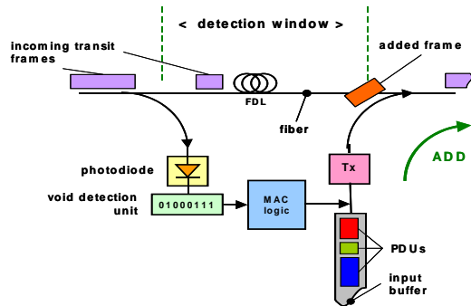
Fig. 2. Schema of the CSMA/CA based MAC.
