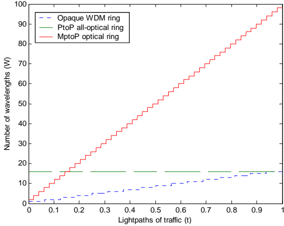
Fig. 9. The number of required wavelengths in the WDM ring networks.
