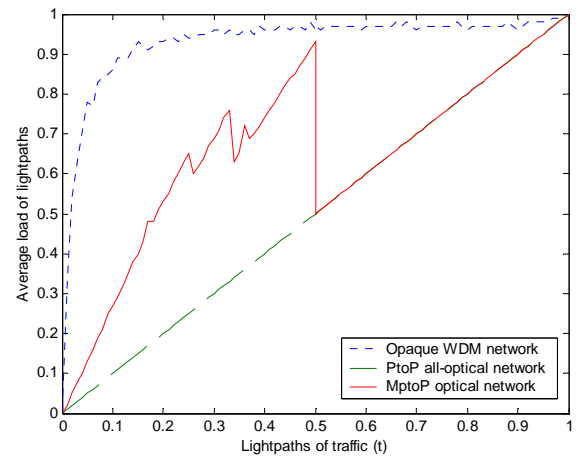
Fig. 20. The average wavelength utilisation in the US backbone.
