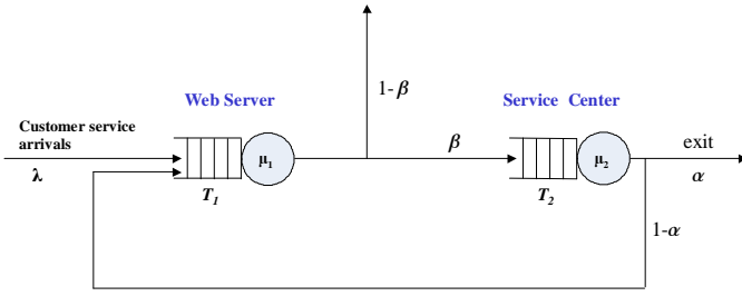
Fig. 2. A Queueing Performance Model for Computer Services in Cloud Computing
