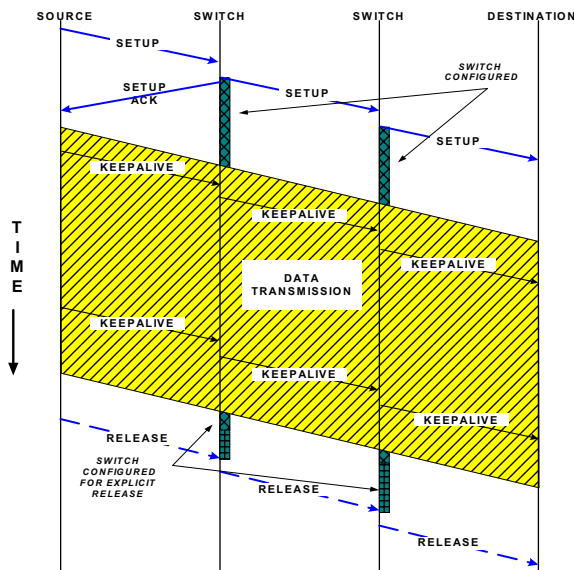
Figure 1. Optical data transmission with SETUP , KEEPALIVE , and RELEASE control messages
