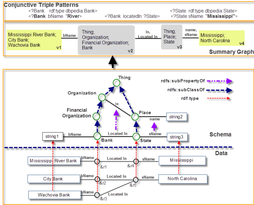
Fig. 1. Graph Summarization
