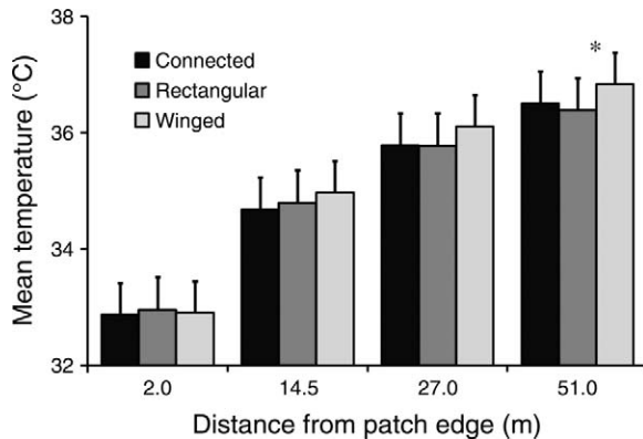
FIG. 3. Temperature (mean + SE, from readings taken between 07:00 and 19:00 hours) increased with increased distance from patch edge. At the farthest distance (51 m), temperature was significantly higher in winged patches than in rectangular patches.
