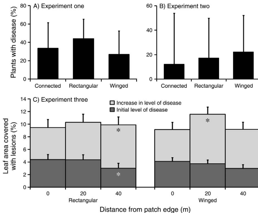
FIG. 2. (a) In experiment one, disease dispersal and development throughout an entire growing season resulted in a significantly higher percentage (mean + SE) of diseased plants in rectangular than in winged patches, but no significant differences between connected patches and either winged or rectangular patches. (b) In experiment two, we found no significant effect of connectivity or patch shape on where spores dispersed (mean + SE). (c) In experiment three, levels of disease, measured as the percentage of leaf area covered by disease lesions (mean + SE), differed at initial levels (dark fill) only in rectangular patches (left-hand columns), where plants 40 m from the edge had significantly lower initial levels of disease than plants 0 or 20 m from the edge; for winged patches (right-hand columns), there were no significant differences in initial levels of disease. There was significantly higher disease development (light fill) in rectangular plots for plants 40 m from the edge, and in winged plots for plants 20 m from the edge vs. 0 m from the edge.
