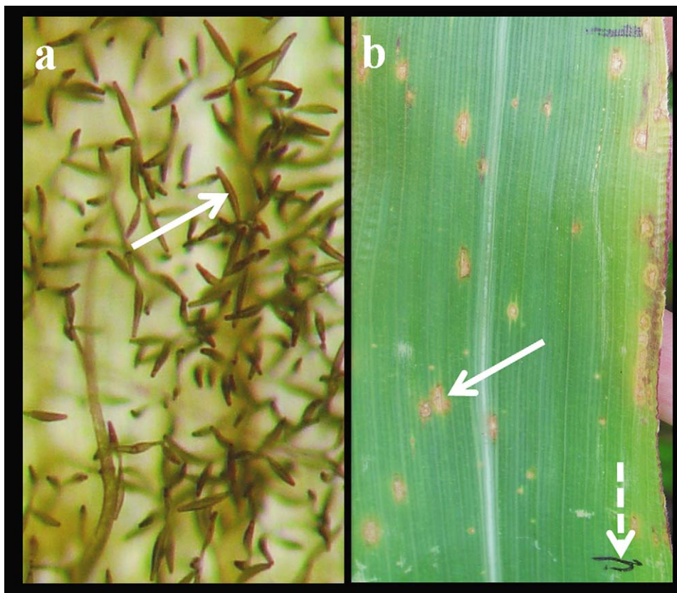
PLATE 1. Spores and lesions of southern corn leaf blight ( Bipolaris maydis ). (a) Spores of southern corn leaf blight are easily distinguished under microscopy. (b) Southern corn leaf blight creates distinct lesions on the corn leaf (solid arrow). In experiment three, four-inch sections (1 inch = 2.54 cm) were marked on the leaf surface to delineate areas in which to monitor disease development (dashed arrow). Photo credit: Brenda Johnson.
