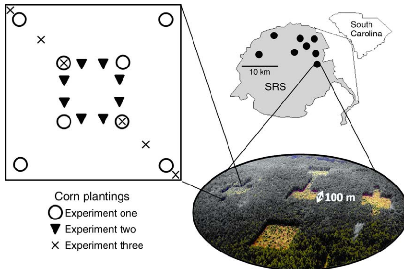
FIG. 1. Experiment at the Savannah River Site, South Carolina, USA. Each of eight blocks (black circles in the SRS map) is composed of five habitat patches with a 100 \times 100 m center patch and one surrounding patch connected by a linear habitat corridor. The other three surrounding habitat patches are of two types: rectangular patches control for the increase in habitat area that is a by-product of corridor addition and have the area of a corridor added onto a square habitat patch, and winged patches control for the increase in both habitat area and edge and have two 75-m dead-end “corridors” on either side of a square patch. Habitat patches are regenerating longleaf pine ( Pinus palustris ) savannah cut into a pine plantation matrix. Habitat edges are distinct transitions between the savannah-like patches and 25 m tall pine plantation. The inset shows the placement of corn ( Zea mays ) plants for each of the three experiments (with each symbol representing an individual corn plant). Photo credit: Ellen Damschen.
