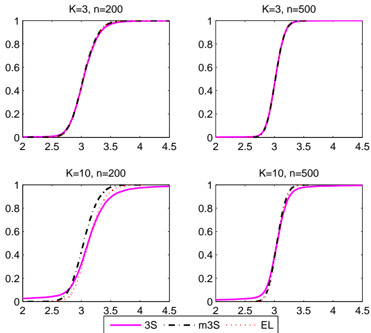
Figure 1: Simulated cumulative distribution function of the 3S, m3S and EL estimators. Design D.
