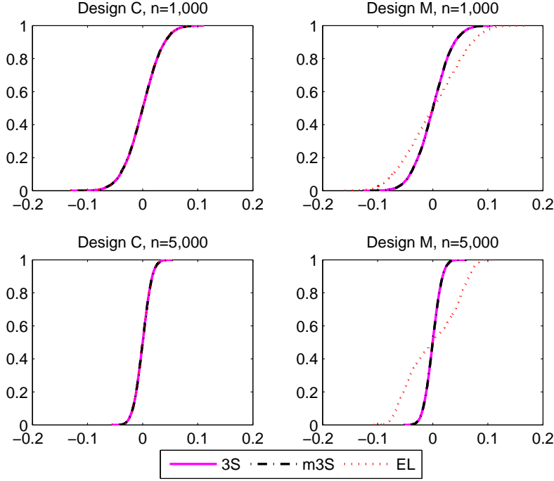
Figure 2: Simulated cumulative distribution function of the 3S, m3S and EL estimators. Well specified vs misspecified models. Designs C and M
