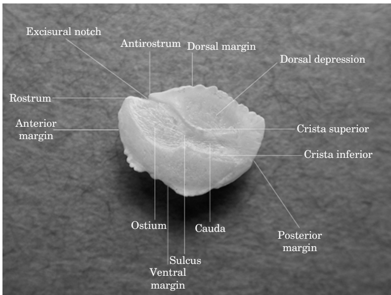
FIG. 5. Mesial view of right sagitta of a male Kurtus gulliveri (185 mm L_S ). This otolith is 8.4 \times 6.3 mm and 1.9 mm thick.
