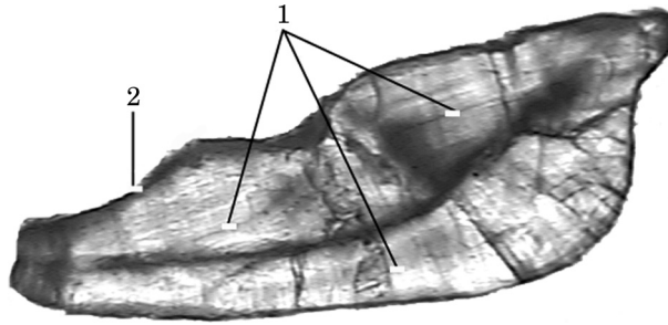
FIG. 4. Sectioned sagitta from a female Kurtus gulliveri (210 mm L_S ). This otolith is 9.3 \times 6.4 mm and 1.95 mm thick. Numbers are annual growth rings.
