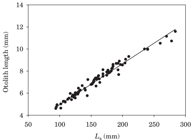
FIG. 6. Plot of otolith and standard lengths. The curve was fitted by eye.
