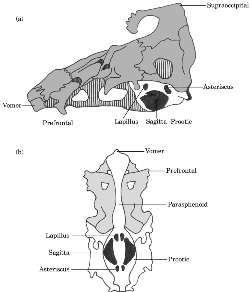
FIG. 2. (a). Lateral view of male Kurtus gulliveri skull showing the location of the three otoliths based on a computed tomography (CT) scan. (b). Ventral view of the skull showing location of the three otoliths. Drawing modified from de Beaufort (1914).
