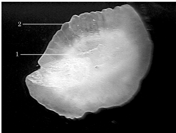
FIG. 3. Whole sagitta showing two annuli from a male Kurtus gulliveri (185 mm L_S ). Numbers are annual growth rings.
