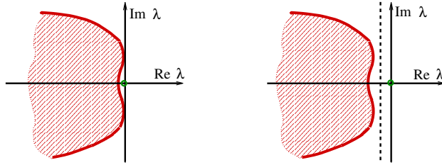
Figure 2: A schematic illustration of the spectrum in the case \alpha = 0 . Weight \rho_\beta opens a gap between the essential spectrum and the imaginary axis by pushing the essential spectrum to the left.
