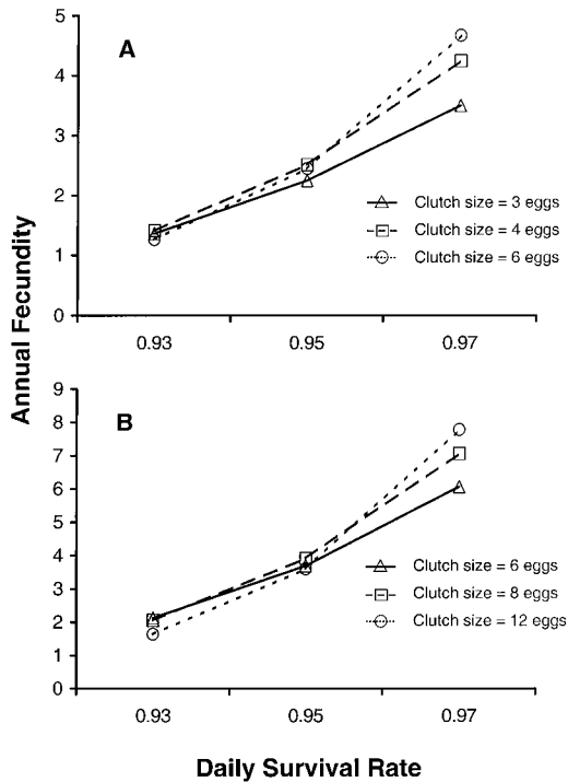
FIG. 3. Annual fecundity versus daily nest survival for different ways to lay a maximum of (A) 12 eggs and (B) 24 eggs. Season length ( t = 90 days), nesting cycle ( L = 25 days), and renesting intervals ( d = 8 and D = 14 days) were held constant. Triangles represent a maximum of m = 4 clutches, squares m = 3 clutches, and circles m = 2 clutches. Annual fecundity is higher for larger clutch sizes as the daily survival of nests increases.
